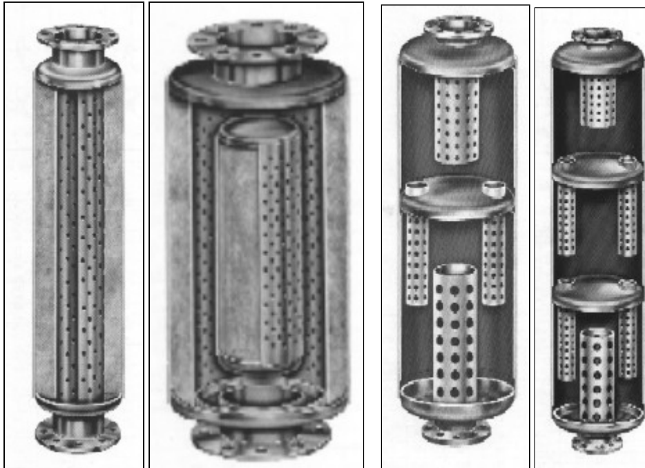
Figure 3 Use absorptive mufflers (left two) for high-frequency noise. Consider expansion chamber or reactive mufflers (right two) for low frequencies.
